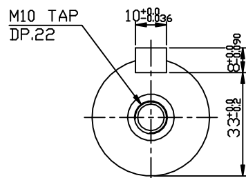
OUTPUT SHAFT
