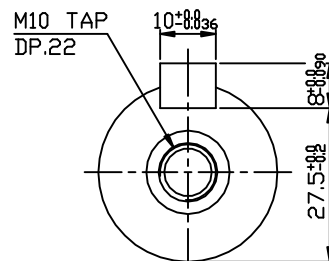
OUTPUT SHAFT
