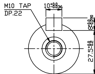
OUTPUT SHAFT
