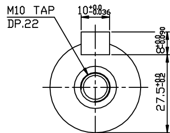
OUTPUT SHAFT
