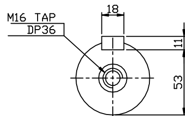
OUTPUT SHAFT
