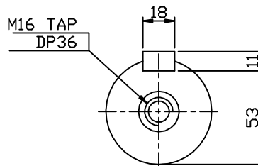
OUTPUT SHAFT
