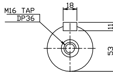
OUTPUT SHAFT
