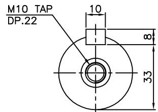
OUTPUT SHAFT
