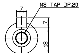
OUTPUT SHAFT
