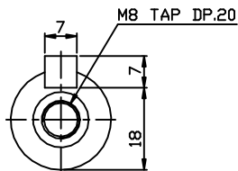
OUTPUT SHAFT
