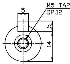
OUTPUT SHAFT
