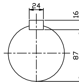
OUTPUT SHAFT
