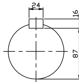
OUTPUT SHAFT
