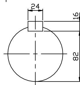
OUTPUT SHAFT
