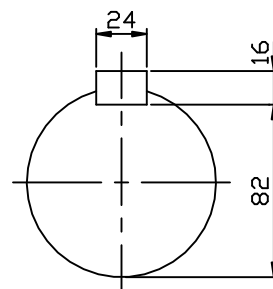
OUTPUT SHAFT
