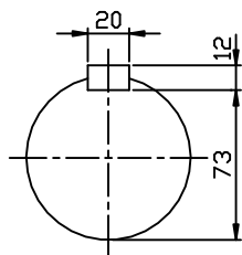
OUTPUT SHAFT
