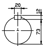
OUTPUT SHAFT
