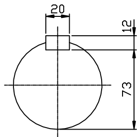
OUTPUT SHAFT
