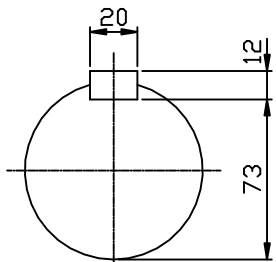
OUTPUT SHAFT
