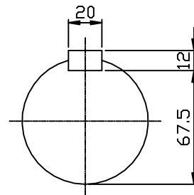
OUTPUT SHAFT
