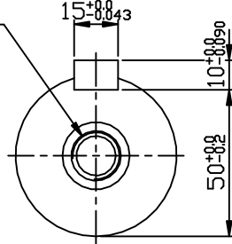
OUTPUT SHAFT
