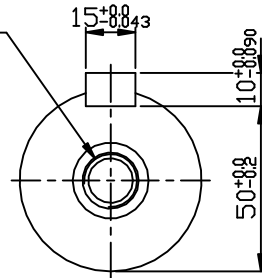
OUTPUT SHAFT
