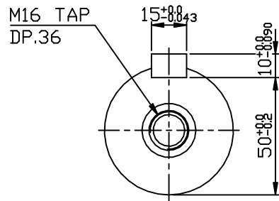
OUTPUT SHAFT
