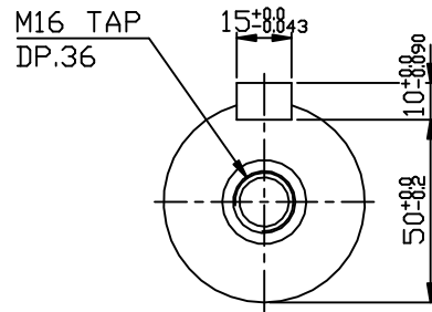
OUTPUT SHAFT
