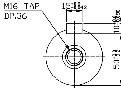
OUTPUT SHAFT
