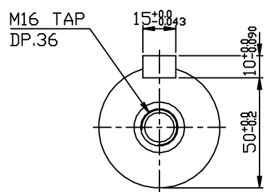
OUTPUT SHAFT
