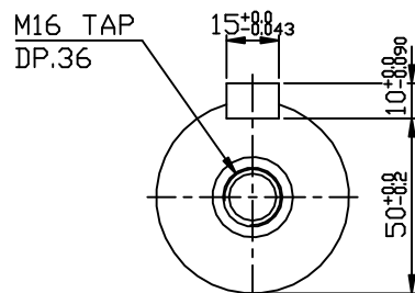
OUTPUT SHAFT
