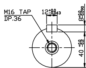
OUTPUT SHAFT
