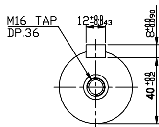
OUTPUT SHAFT
