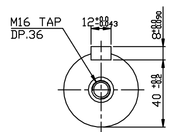
OUTPUT SHAFT
