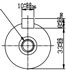
OUTPUT SHAFT
