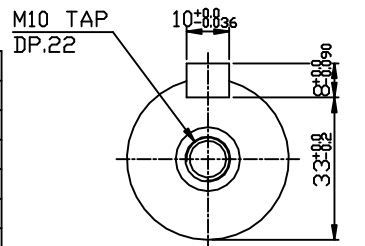
OUTPUT SHAFT
