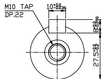
OUTPUT SHAFT
