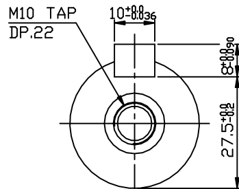
OUTPUT SHAFT
