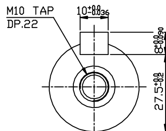
OUTPUT SHAFT
