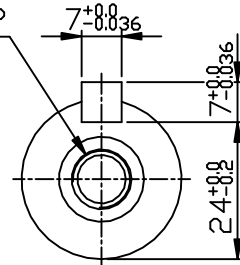
OUTPUT SHAFT
