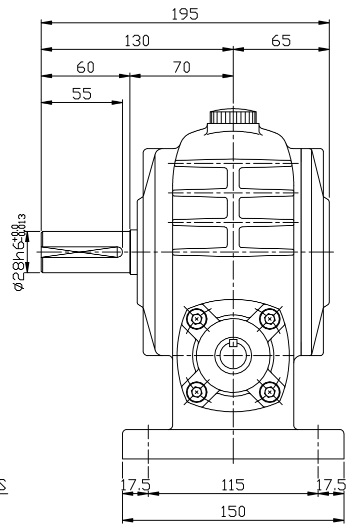
OUTPUT SHAFT
