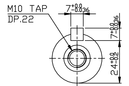
OUTPUT SHAFT
