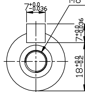
OUTPUT SHAFT
