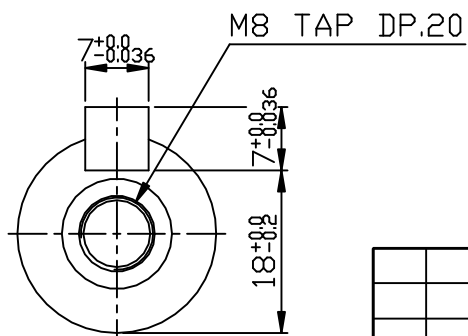
OUTPUT SHAFT
