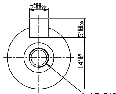
OUTPUT SHAFT
