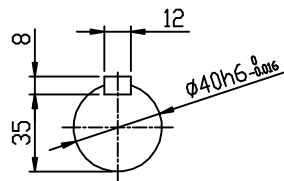
OUTPUT SHAFT
