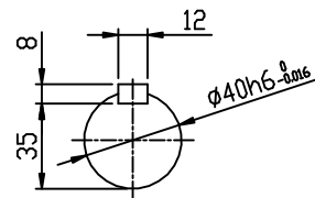
OUTPUT SHAFT
