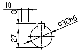
OUTPUT SHAFT
