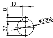
OUTPUT SHAFT
