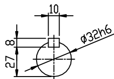
OUTPUT SHAFT
