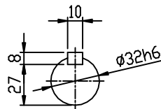
OUTPUT SHAFT
