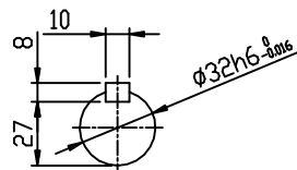
OUTPUT SHAFT
