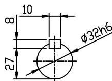
OUTPUT SHAFT
