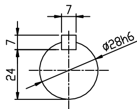
OUTPUT SHAFT
