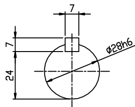
OUTPUT SHAFT
